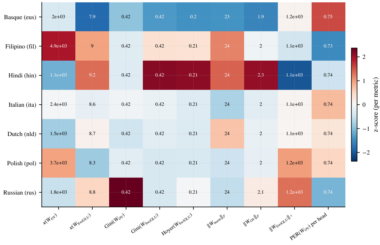
Q1a · Final-step interpretability across L1 (B1 balanced, FineWeb-100M)
